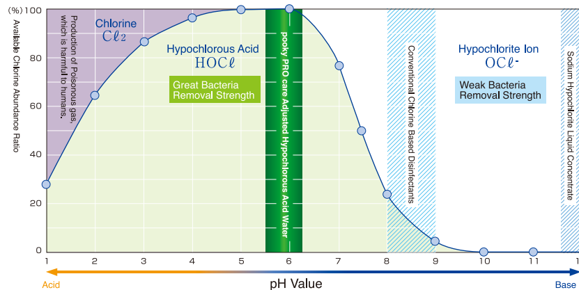
Abundance Ratio of Free Available Chlorine Through Formation Principle and [pH] Transformation
